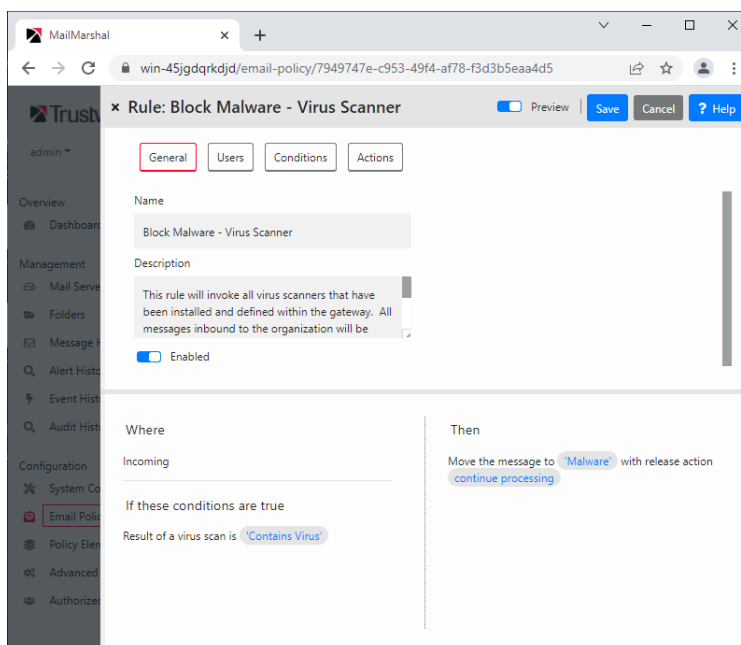
Figure 1: Enabling Rules
