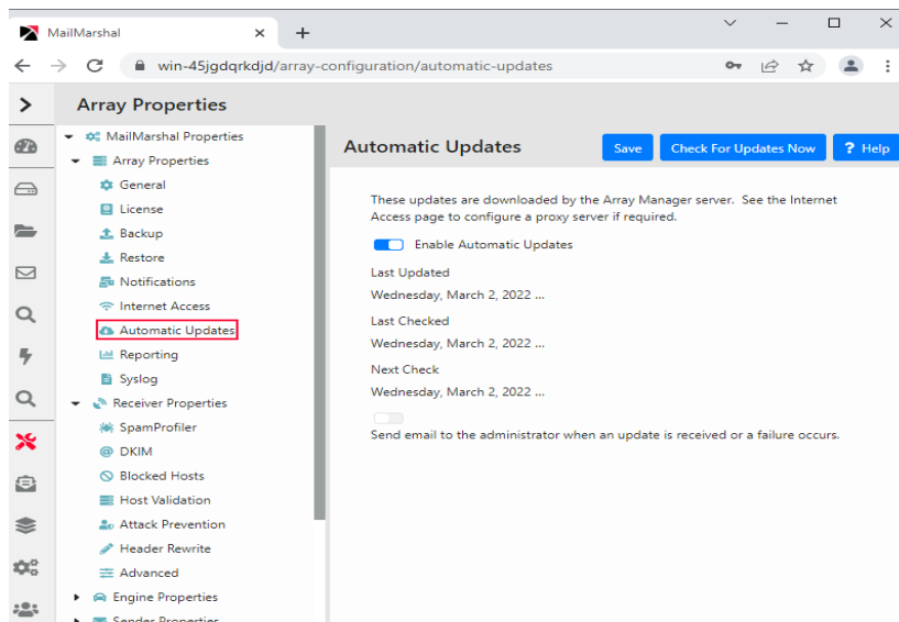
Figure 5: MailMarshal Properties
